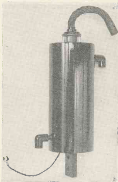
Fig. 2 Type BK24 steel Ignitron (diameter 4 in.).
