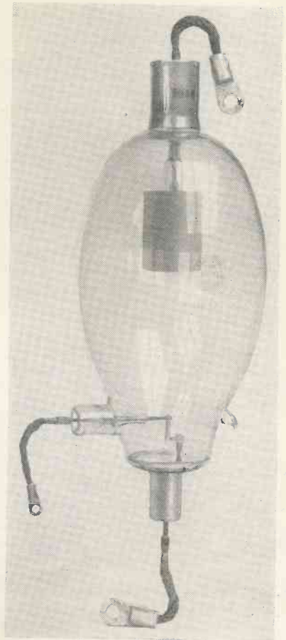
Fig. 1. Type BK22 Ignitron (diameter 7½ in.).
