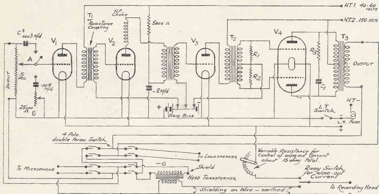
Fig. 8. Circuit diagram of amplifier including switching arrangement.
