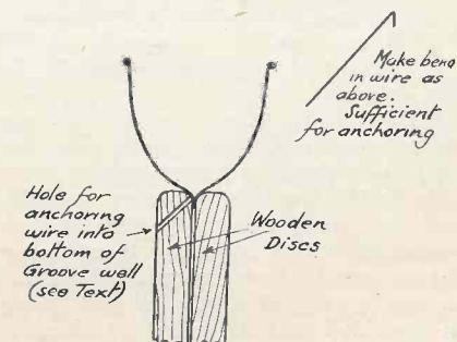
Fig. 6. Sectional view of drum groove showing method of anchoring wire.
