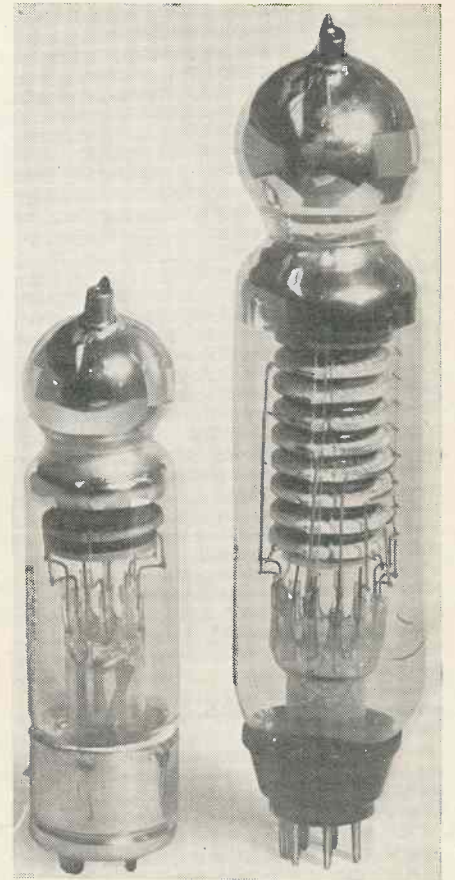
Photograph of two-stage and ten-stage Photo-Augetrons.
