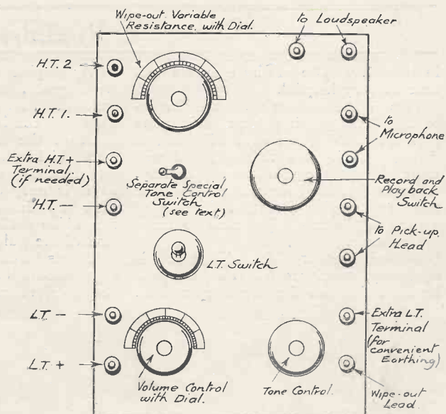
Fig. 7. Diagram showing arrangement of terminals and controls on the amplifier panel.
